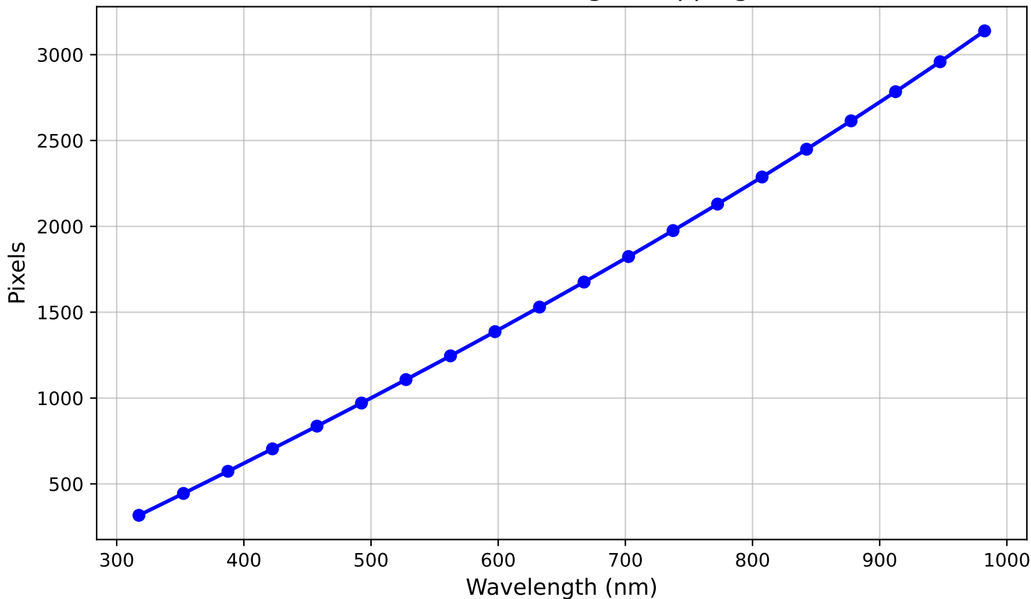
Pixel to Wavelength Mapping
